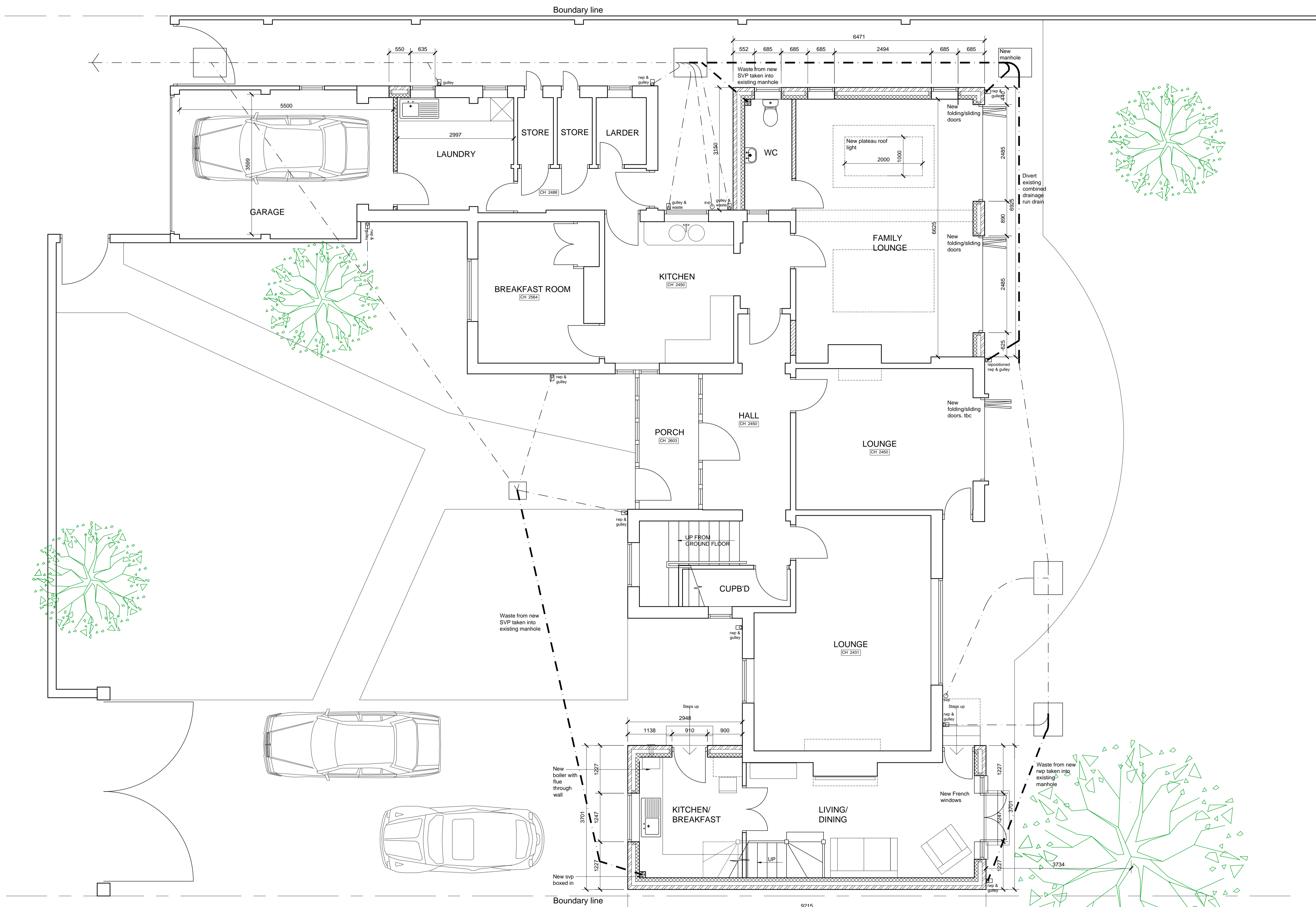
PROPOSED GROUND FLOOR LAYOUT
